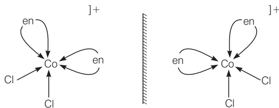
Non-superimposable isomers of [\text{Co(en)}_2\text{Cl}_2]^+
