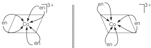
Non-superimposable isomers of [\text{Co(en)}_3]^{3+}
